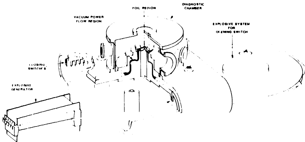
Fig. 1. Pioneer I foil implosion system.
